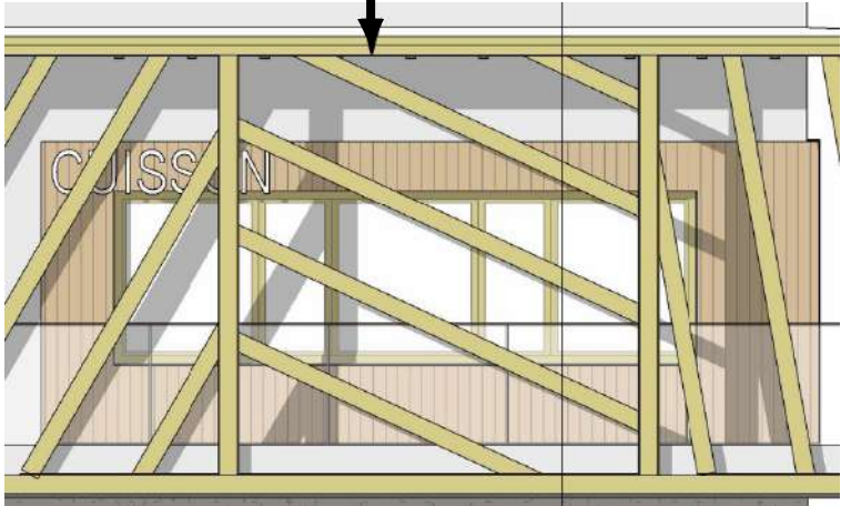
FACADE SUD
