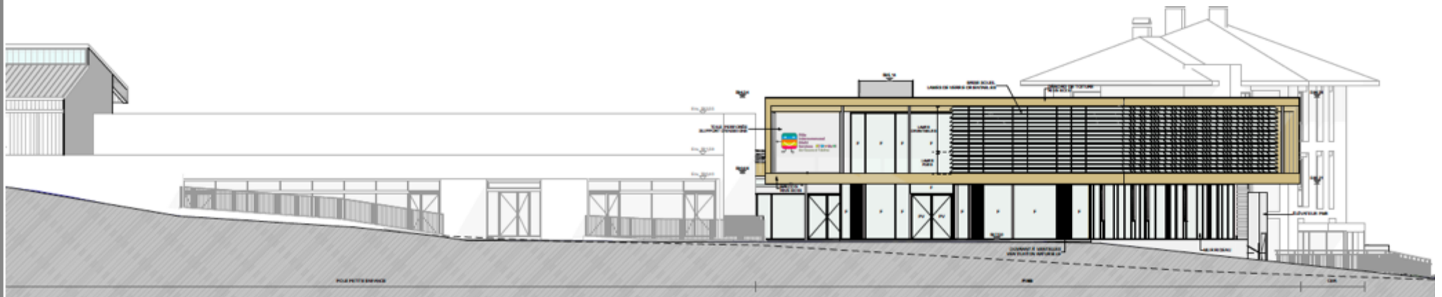
FACADE SUD
